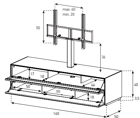
FLOOR CABINETS 160 x 40 CM (WITHOUT HOLE) EX32F (Adjustable shelf + 4 cm)
