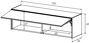
ED61TS / PS (WITH CABLE MANAGEMENT)
