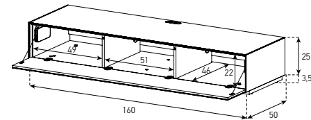
160 x 25 CM (WITH HOLE & BRACKET) EX36F
