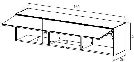
ED31F (WITH CABLE MANAGEMENT)
